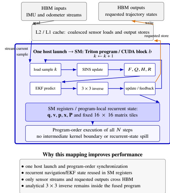
Fig. 4 Correspondence between the Triton whole-scan operator and the GPU memory hierarchy. Sensor samples and requested outputs are streamed through HBM and cache, while one CUDA block executes the ordered trajectory scan and retains recurrent navigation and EKF state in SM registers. This mapping reduces dispatch, synchronization, and global-memory traffic on the latency-bound critical path.
